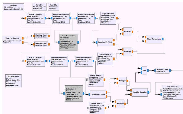
Figure 2: GNURadio screenshot of the car audio modulation system.
