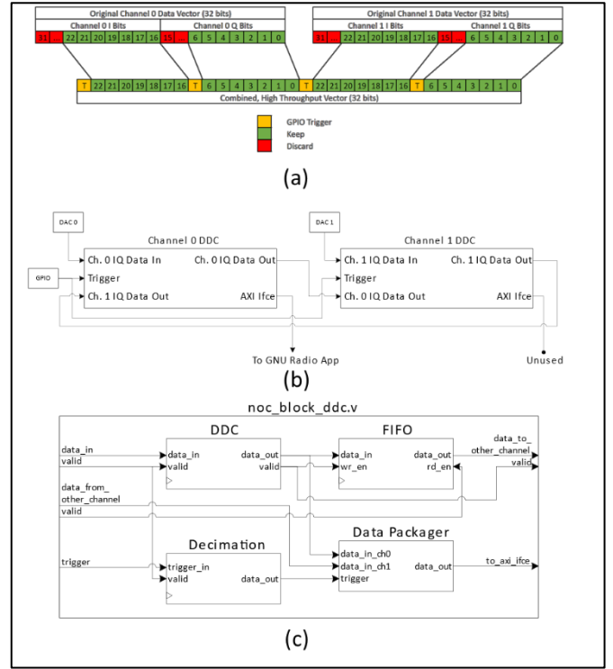
Figure 9. Implementation of the new FPGA data format and trigger signal incorporation.
